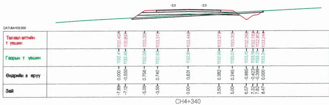
CH4+340
