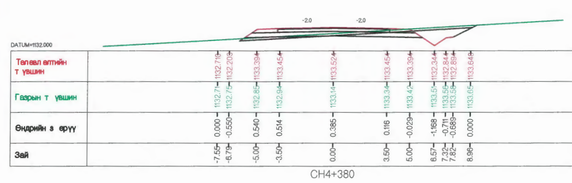
CH4+380
