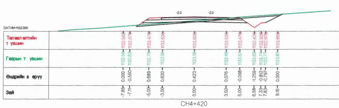
CH4+420
