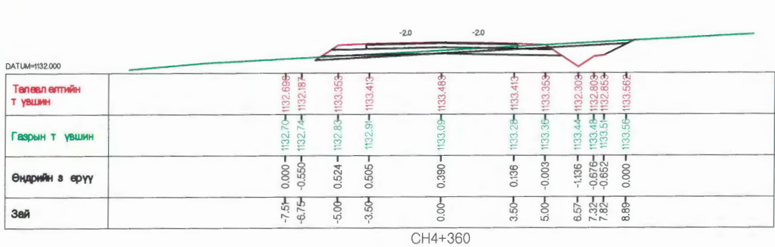
CH4+360
