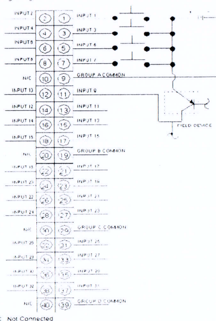
Wiring Diagram
