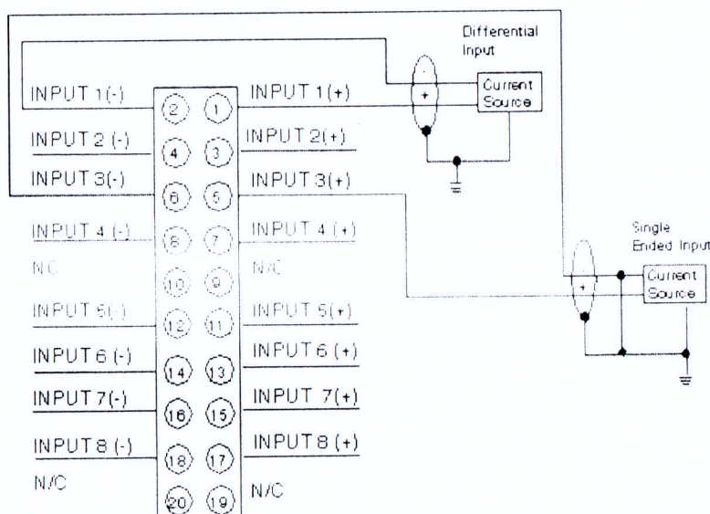
Wiring Diagram
