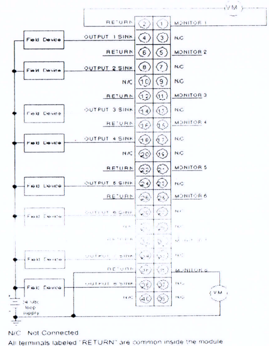
Wiring Diagram
