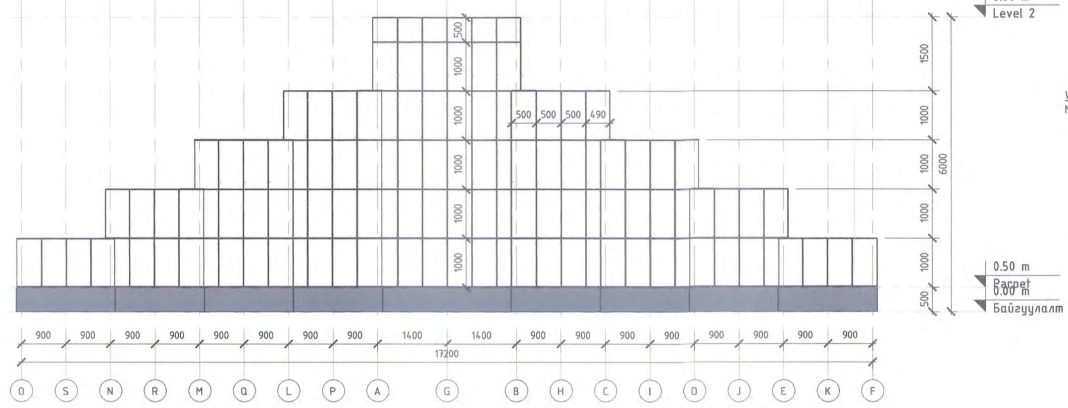
South M:1:75
