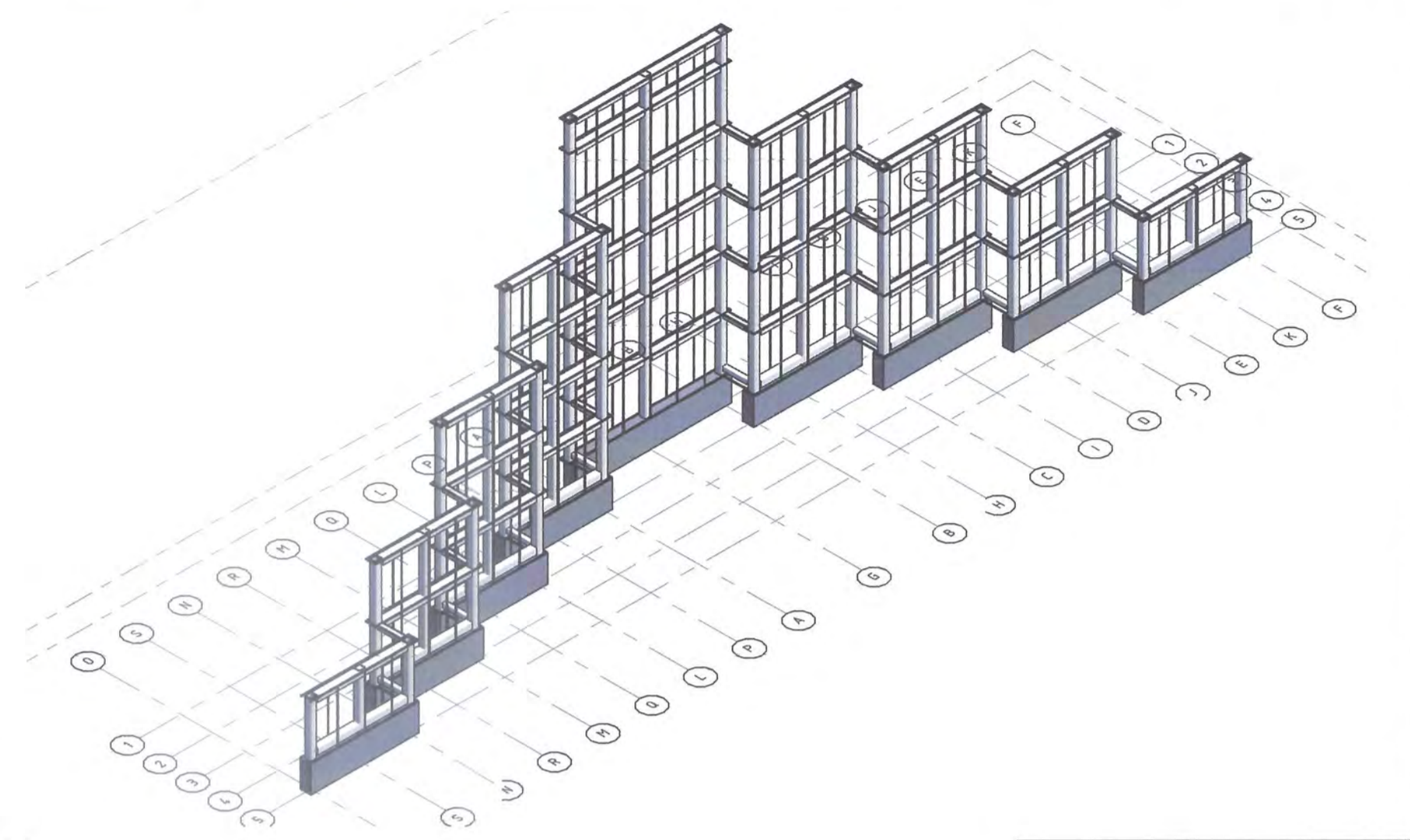
West M:1:75
