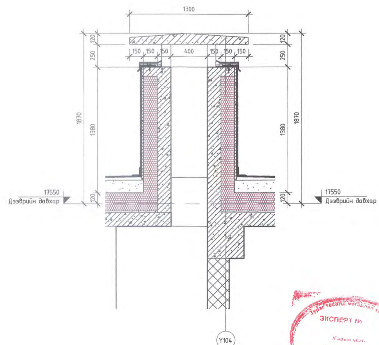
5 Section 4-4 - Callout 1 M: 1 : 25
