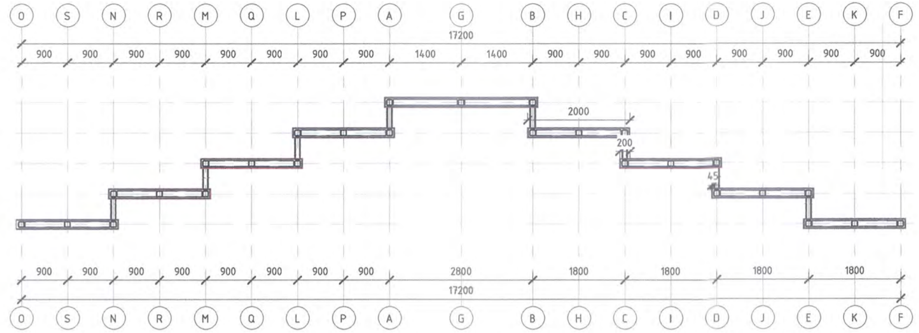
South M:1:75
