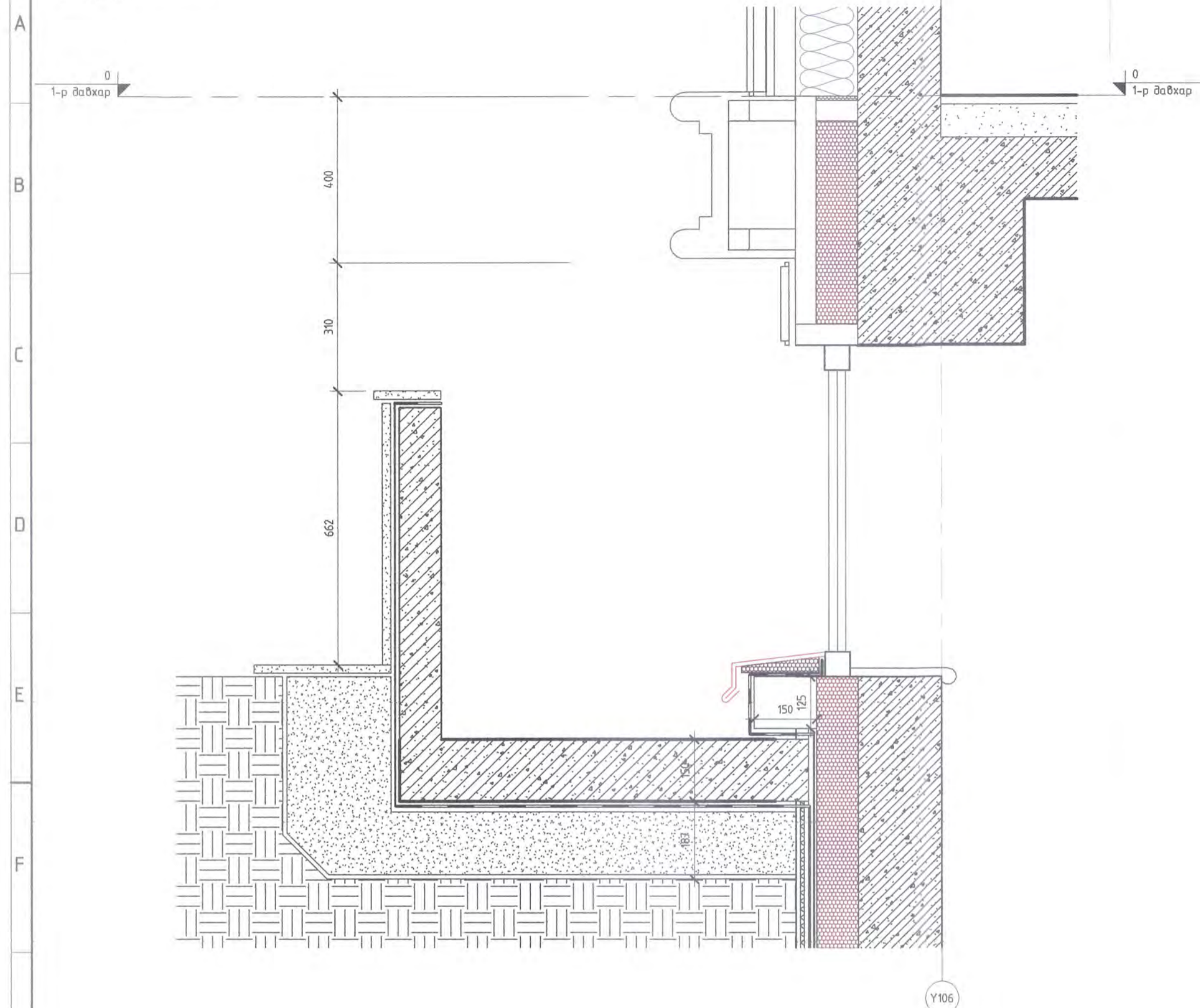
3 Section 4-4 - Callout 2 M: 1 : 10
