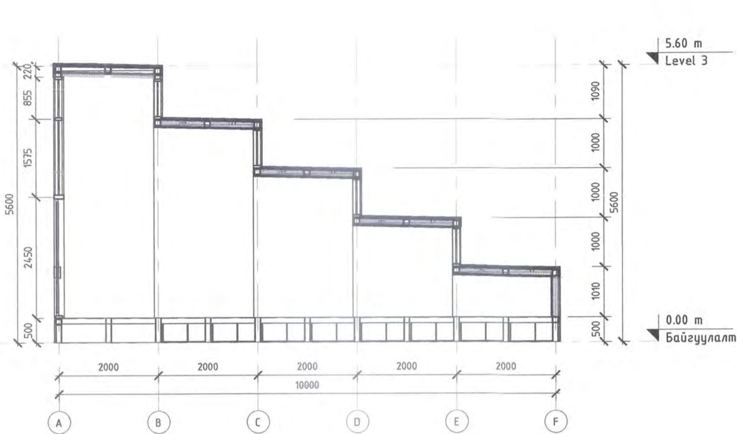
North M:1 : 75
