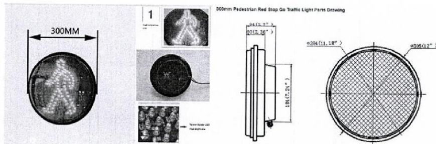
300mm Pedestrian Red Stop Go Traffic Light Parts
